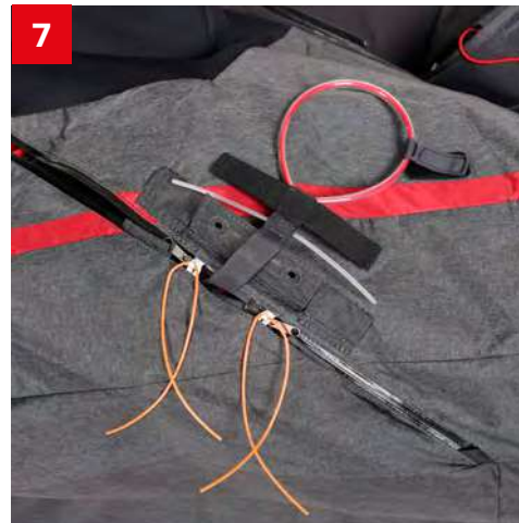
7 Pass the parachord into the bottom fabric loops
